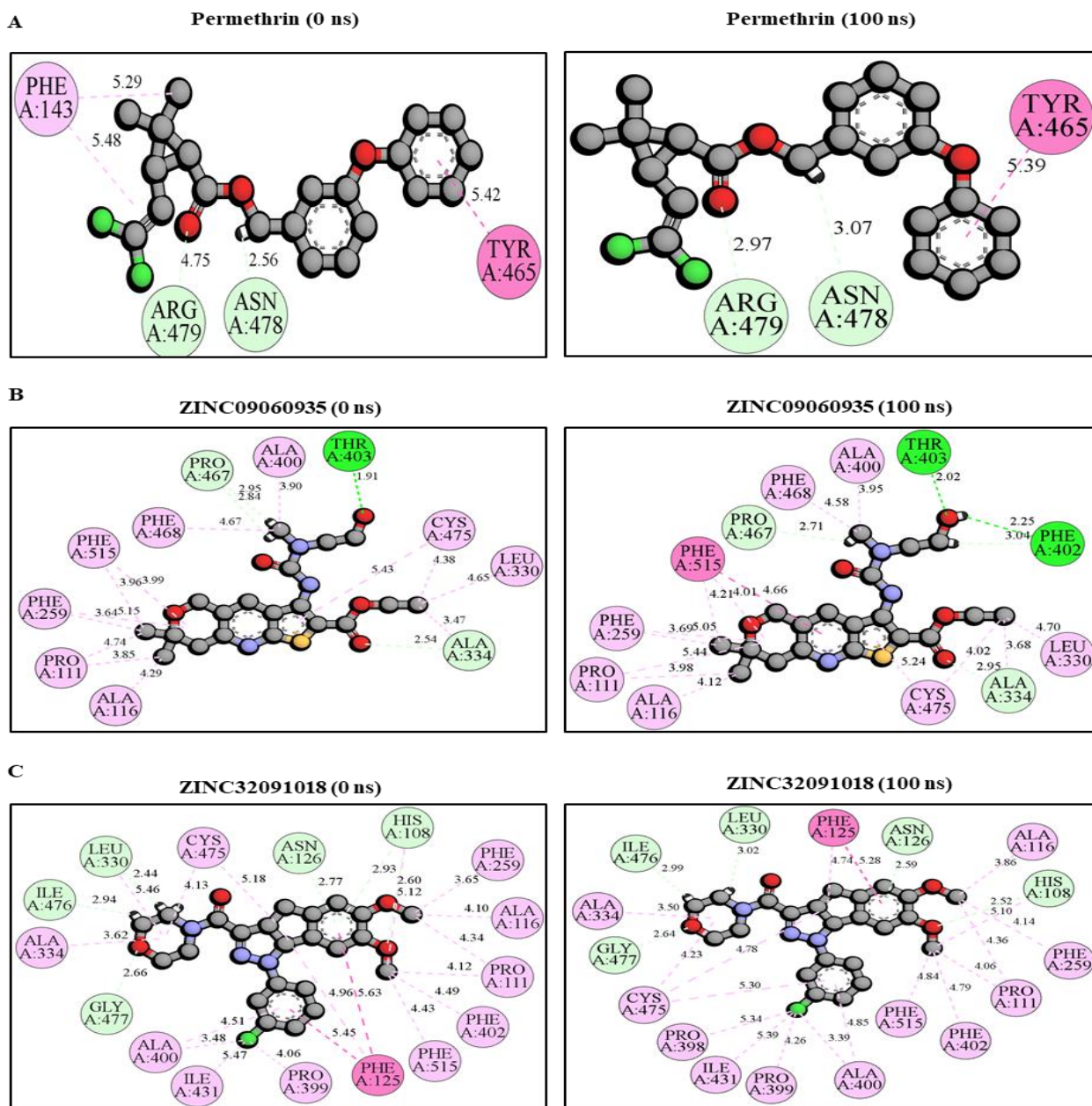
Fig. 5. Time-dependent distance and interaction analysis of CYP9e2 complexes with permethrin, ZINC09060935, and ZINC32091018. (A) The interaction and distance between permethrin and CYP9e2 residues over time, depicted at initial conformation (0 ns), and final 100 ns. (B-C) The interaction and distance between the top hits ZINC09060935 and ZINC32091018 over the same time points. Dark green residues have a conventional hydrogen bond, whereas light green residues have a carbon-hydrogen bond, pink (Pi-alkyl), and dark pink (Pi-pi stacked) bonds.
