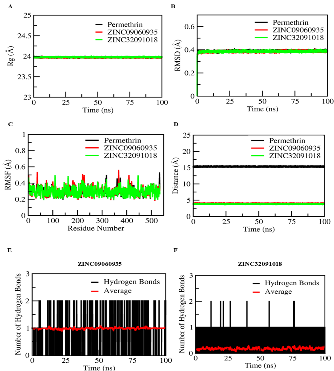
Fig. 6. Trajectory analysis of CYP9e2 complexes with Permethrin, ZINC09060935, and ZINC32091018. (A) The Radius of gyration (Rg). (B) The Root-mean-square deviation (RMSD). (C) Root-mean-square fluctuation (RMSF). (D) The distances between the CYP9e2, permethrin, ZINC09060935, and ZINC32091018. (E-F) The number of hydrogen bonds.
