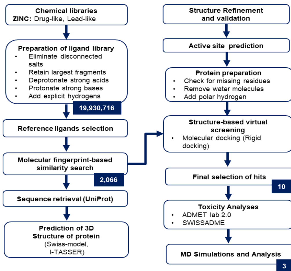
Fig. 1. The overall summary of the virtual screening workflow for the identification of lead compounds. The dark-blue boxes indicate the number of ligands carried forward into the next level.
