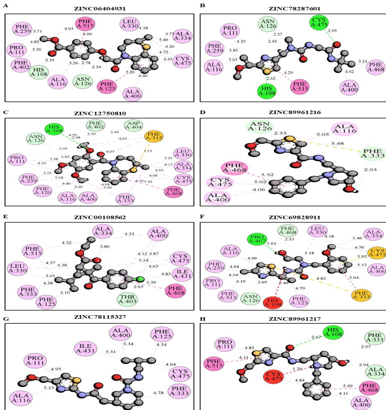
Fig. 3. Distance and interaction analysis of top hits with CYP9e2. (A-H) The interaction and distance between top hits and CYP9e2 residues. Dark green residues have a conventional hydrogen bond, whereas light green residues have a carbon-hydrogen bond, pink (Pi-alkyl), dark pink (Pi-pi stacked), purple (Pi-sigma), red (unfavorable donor-donor), and orange (Pi-anion) bonds.
