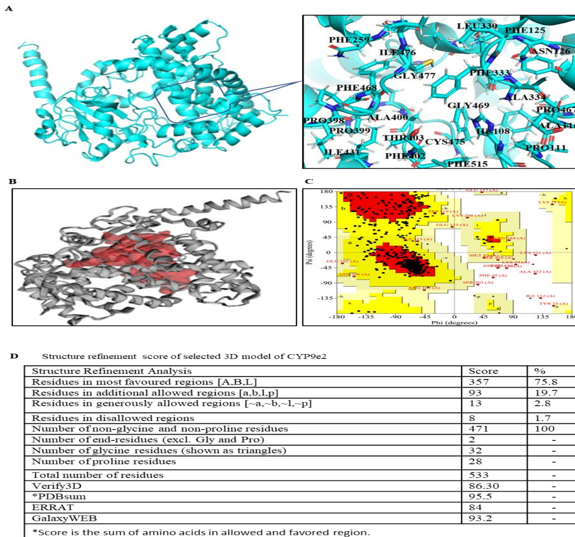
Fig. 2. Prediction and evaluation of the Homology model. (A) Predicted structure and pocket residues representation of CYP9E2. (B) Representation of CYP9E2 active site (red color) using MOE, and CastP server. (C) RAMPAGE analysis of the target protein. (D) Structure refinement score of the selected 3D model of CYP9E2.
