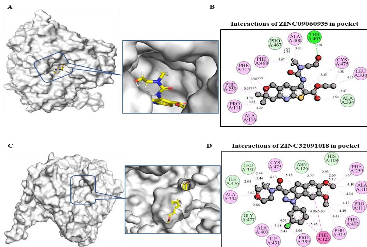
Fig. 4. Interactions of hit compounds with CYP9e2. (A) Surface representation of the receptor and binding pocket of ZINC09060935. (B) A detailed interaction of the key residues within 5 Å of ZINC09060935. (C) Surface representation of the receptor and binding pocket of ZINC32091018. (D) A detailed interaction of the key residues within 5 Å of ZINC32091018.
