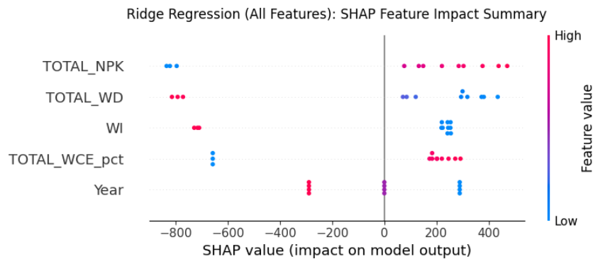
Fig. 3a: SHAP feature impact summary (beeswarm plot) illustrating influence of management inputs on maize yield.
