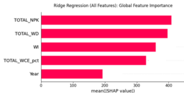
Fig. 3b: Global feature importance of agronomic predictors on maize yield based on regularized Ridge Regression.
