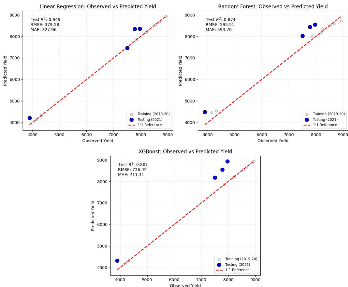
Fig. 1: Comparison of machine learning models for grain yield \text{kg ha}^{-1} (top) prediction using observed vs. predicted scatter plots with a 1:1 reference line.
