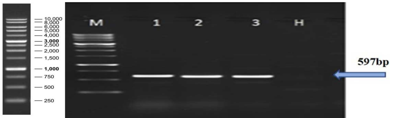
Figure 3: Agarose gel electrophoresis 1% of RT-PCR amplification of a 597 bp fragment using the specific primer for CABYV-CP gene. Lane M represents 1 KB DNA Ladder Gene Direx. The amplified product is 597 bp. Lanes 1, 2 show fragments from infected cucumber and lane 3 shows fragments from infected squash plants collected from the Al-Kharj region. No RT-PCR amplification was observed in uninfected sample cucumber tissue (lane H) as a negative control.
