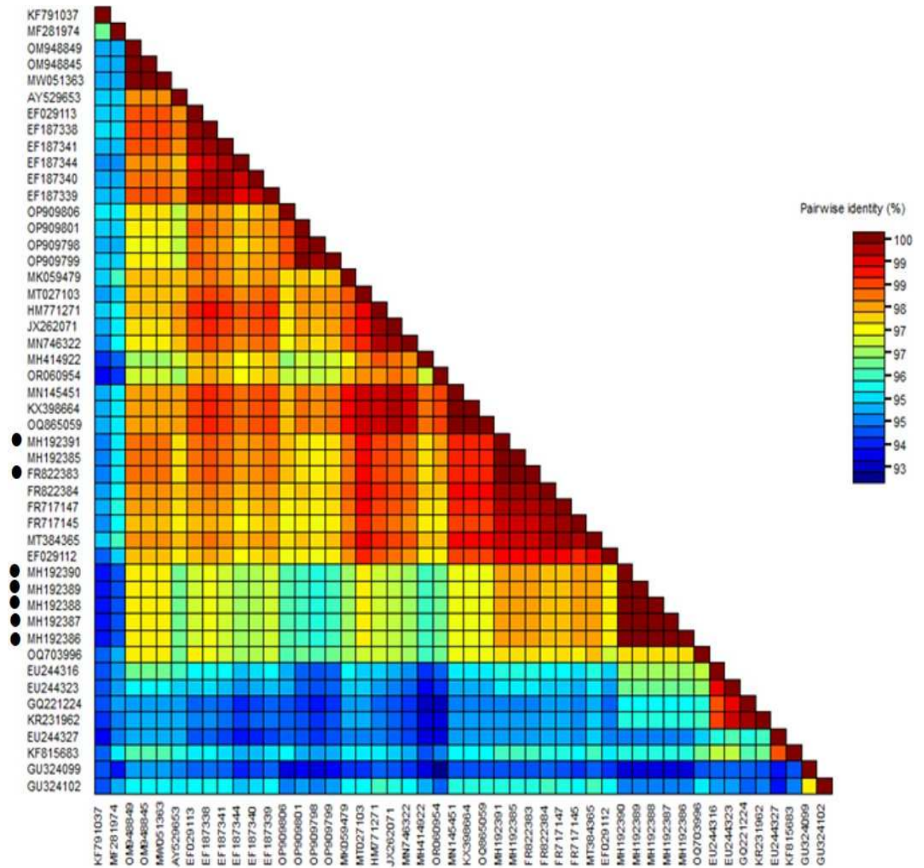
Figure 6. Distance matrix illustrating, the pairwise nucleotide identity percentage of CABYV Saudi isolates as compared with other retrieved isolates from GenBank globally.
