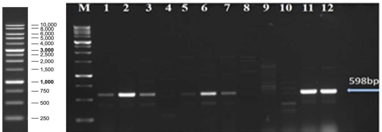
Figure 4: Agarose gel electrophoresis 1% of RT-PCR amplification of a 598 bp fragment using the specific primer for CABYV-CP gene. Amplified products from symptomatic and asymptomatic arable weeds including M. parviflora (Lane 1,2), Ch. murale (Lane 3,4,5), and S. nigrum (Lane 6,7,8,9,10), S. oleraceus (Lane 11,12), No PCR product was amplified from asymptomatic M. parviflora , Ch. murale , S. oleraceus , and S. nigrum collected from Al-Kharj region (lane 4,8,9,10), Lane M represents 1 KB DNA Ladder Gene Direx.
