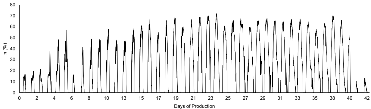
Figure 3. Evaporative cooling efficiency ( \eta ) during the production period
