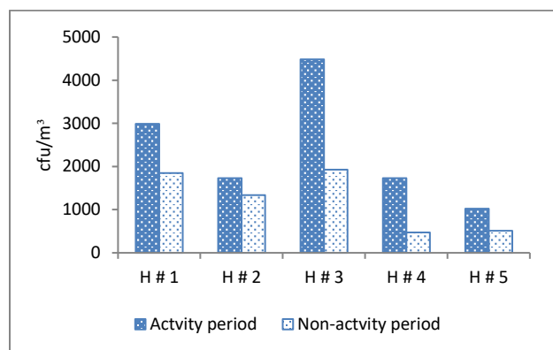
Fig. 1: Levels of bacteria (cfu/m 3 ) in the kitchens during activity and non-activity periods
