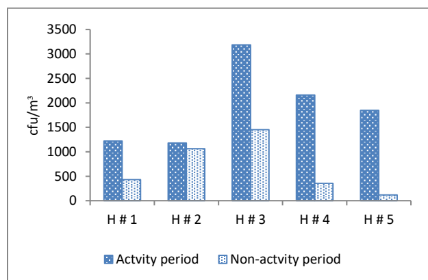
Fig. 2: Levels of bacteria (cfu/m 3 ) in the living room during activity and non-activity periods
