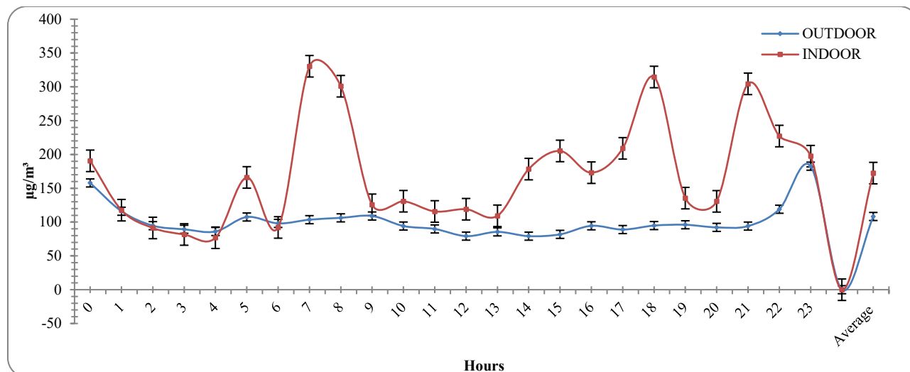
Figure 2: Concentration of fine particles in indoor (low ventilation) and outdoor air
