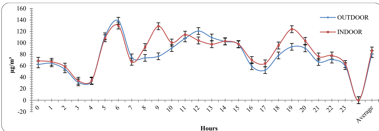
Figure 1: Representative hourly average of indoor and outdoor PM 2.5 under high ventilation scenario
