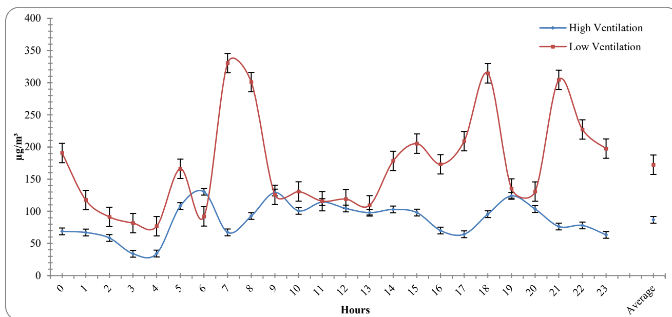
Figure 3: Comparison of Indoor air under high and low ventilation conditions
