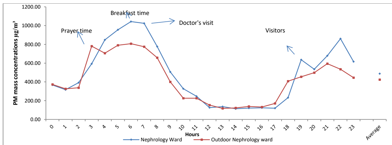
Figure 6: PM 2.5 levels in and out of Nephrology ward resulting from various activities
