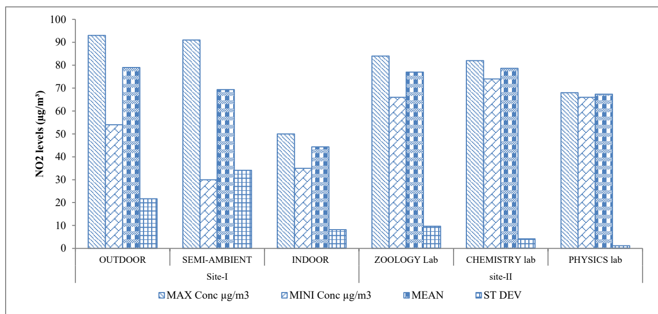
Figure 2 Comparison of mean concentration of NO 2 along with maximum, minimum and standard deviation at two sites.
