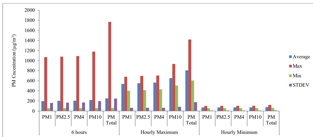
Fig.3. Average, hourly maximum and hourly minimum PM concentrations during the journey from Lahore to Islamabad
