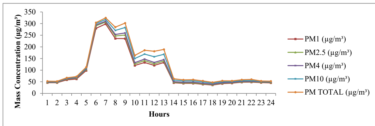
Figure 3: Ambient levels of particulate matter at zero elevation (site A)
