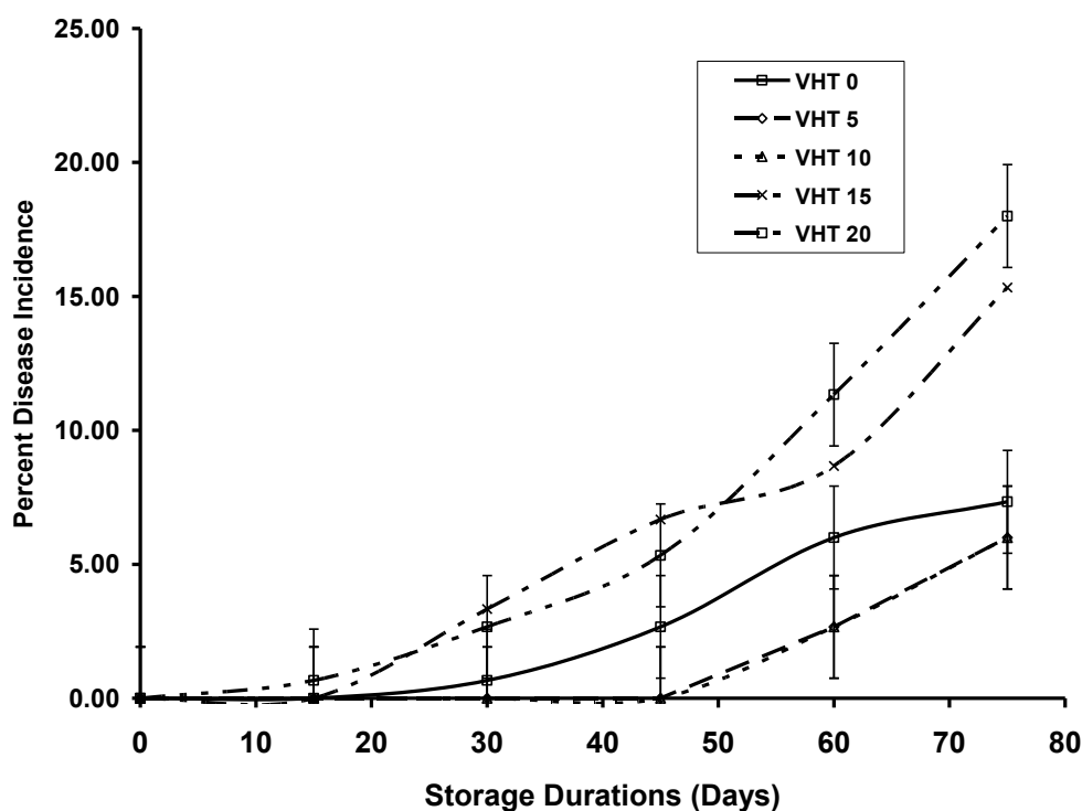
Fig.1(c): Effect of vapor heat treatments on disease incidence in citrus fruits during storage at chilling temperature. The error bars represent LSD at p \leq 0.05 .
