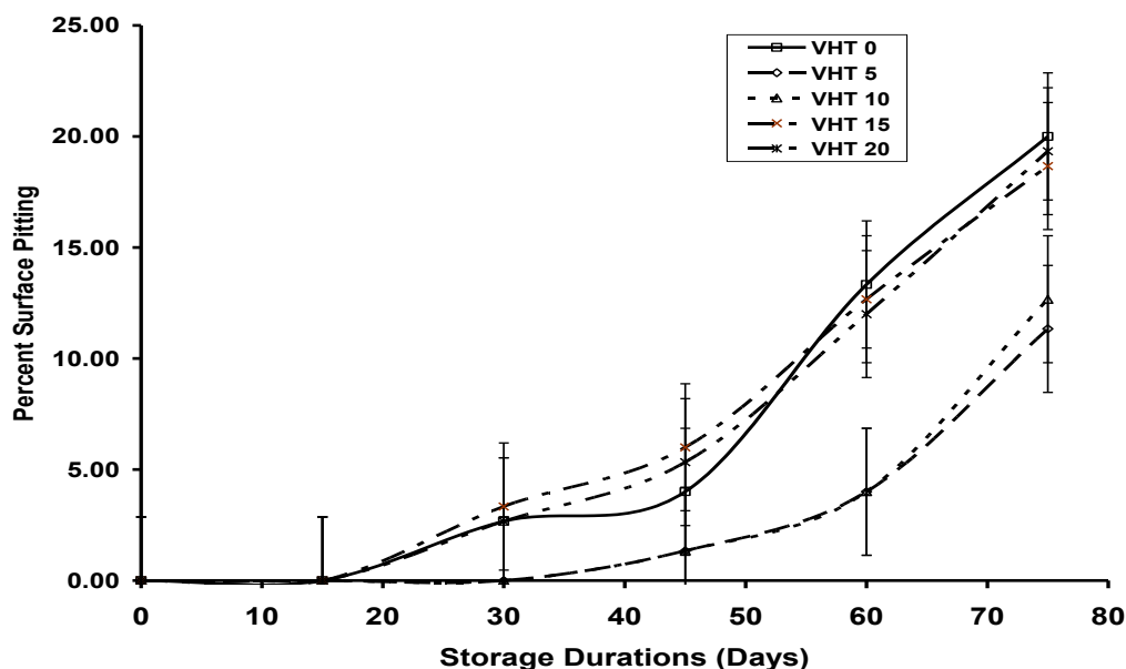
Fig.1 (b): Effect of vapor heat treatments on surface pitting in citrus fruits during storage at chilling temperature. The error bars represent LSD at p \leq 0.05 .
