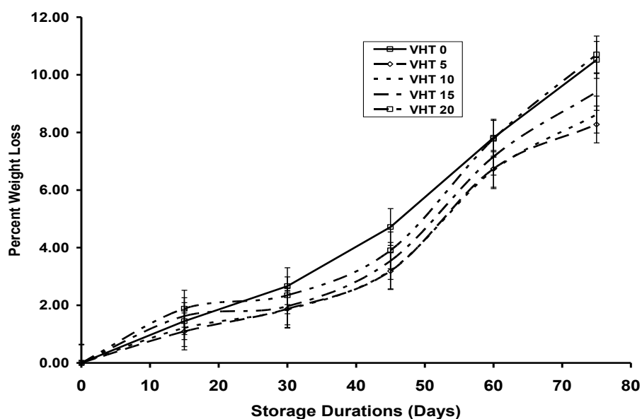
Fig. 1 (a): Effect of vapor heat treatments on weight loss in citrus fruits during storage at chilling temperature. The error bars represent LSD at p \leq 0.05 .
