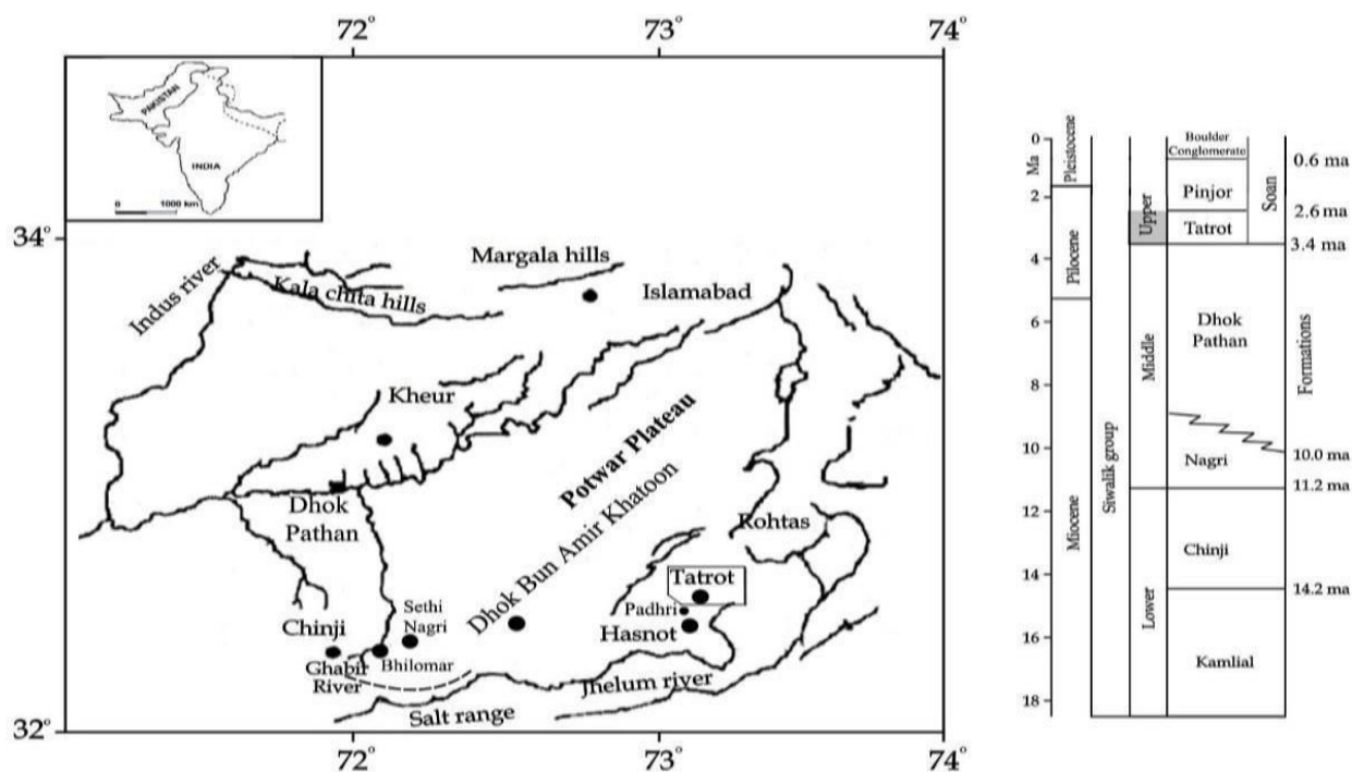
Fig. 1: A Map of the Potwar Plateau which showing the stratigraphic sections and study area of the Upper Siwaliks, Pakistan (Behrensmeyer and Barry, 2005; Nanda, 2008) and the boundary dates are from Dennell et al. (2006).
