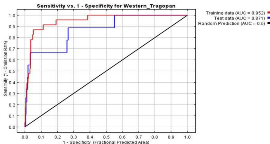
Figure 5: The ROC curve for the training and test data
