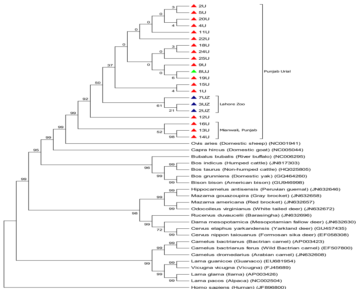
Figure 2: UPGMA Tree constructed with MEGA6 using mitochondrial ATPase6 & ATPase8 genes sequences from Punjab Urial and NCBI reported mammalian sequences.
