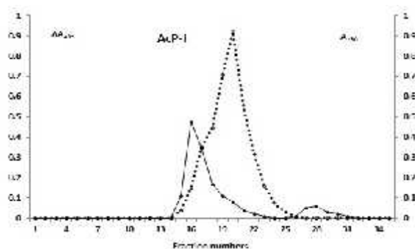
Fig. 4. Optimum pH of acid phosphatase from leaves of v. radiata .
