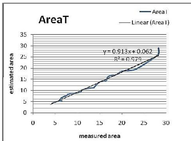
Figure 3. The relationship between leaf area measured with millimeter graph paper (x) and total leaf area estimated using triangle dimensions(y). Total leaf area (Eq.2).
