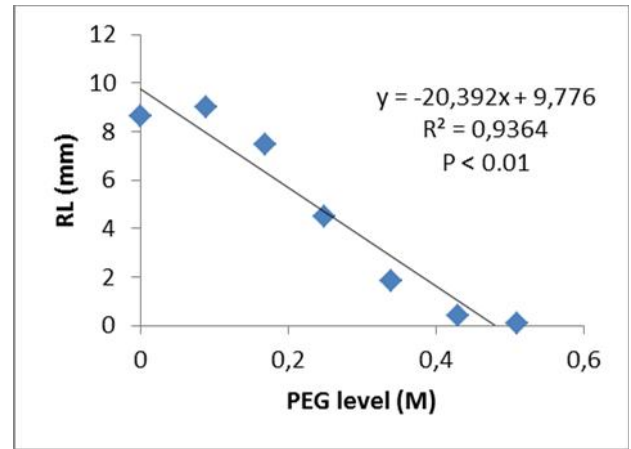
Figure 4. Regression graph showing relationship between PEG level and root length (RL)
