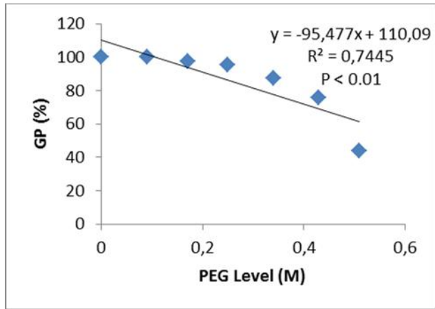
Figure 2. Regression graph showing relationship between PEG level and germination power (GP)
