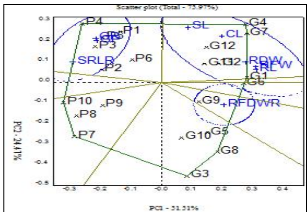
Figure 5. GGE biplot of the relationships between genotype and traits under drought stress
