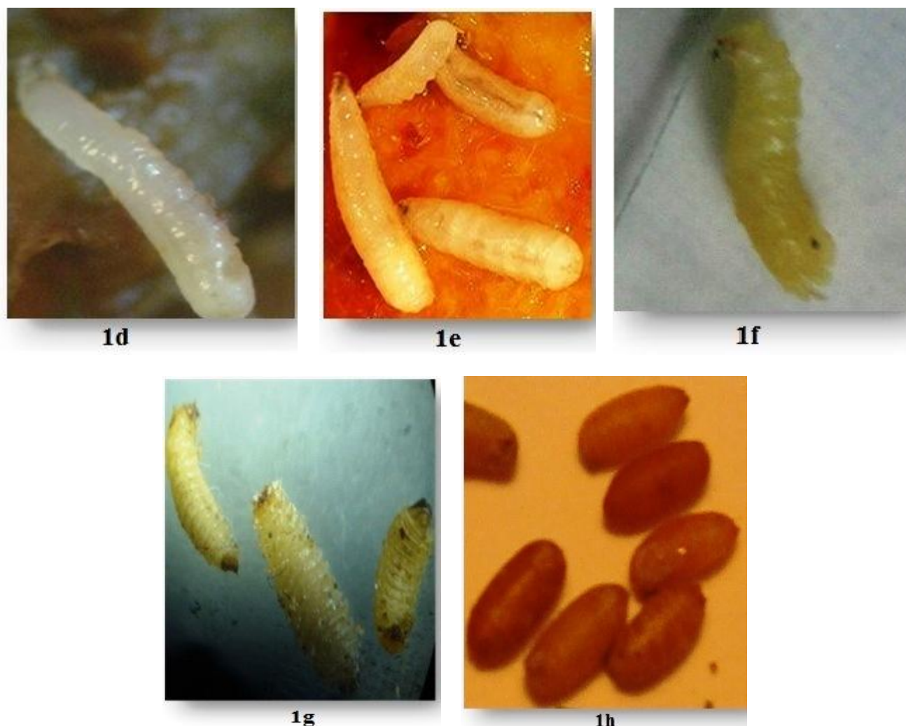
Figure 1. Bactrocera dorsalis (Hendel); 1a, male; 1b, female; 1c, eggs; 1d, 1 st instar; 2 nd instar; 3 rd instar; 1g, Pre-pupal; 1h, Pupae.
